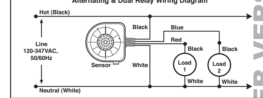
Alternating & Dual Relay Wiring Diagram
