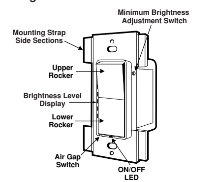
Figure 1 – Dimmer Functions
