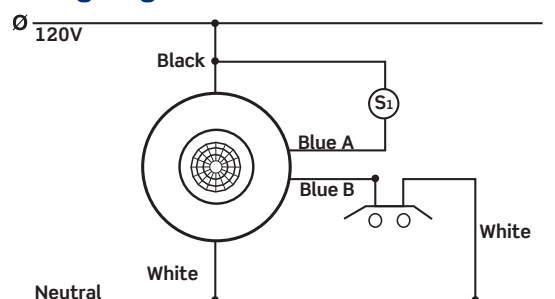
ODCOS-I1 Wiring Diagram with optional switch for override to OFF * Same wiring for all voltages.
