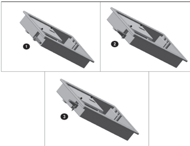
Figure 4 - Flush Mount Enclosure Installation
