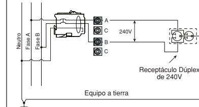
Dia. 1 2 polos, 2 alambres 120/240 VCA
