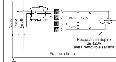
Dia. 2 2 polos, 3 alambres 120/240 VCA
