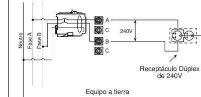
Dia. 1 2 polos, 2 alambres 120/240 VCA
