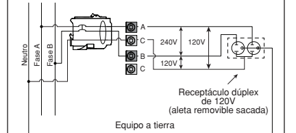
Dia. 2 2 polos, 3 alambres 120/240 VCA
